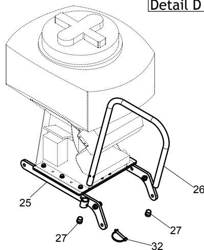
Detail D
