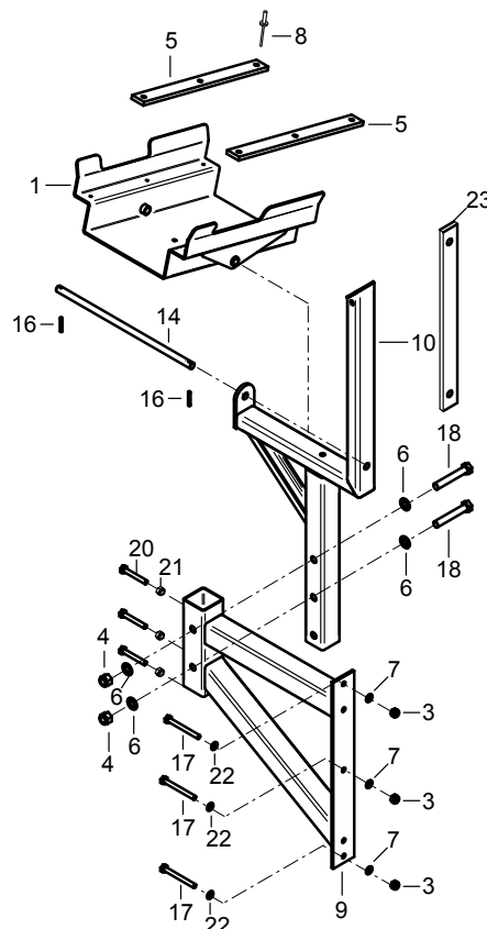
27 - ALA 600 CAMPO E-C-P-R-S
